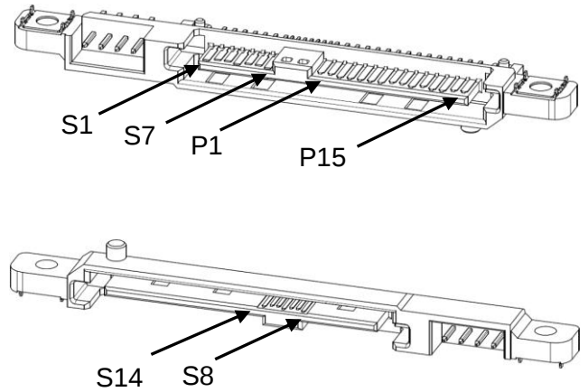
SAS plug connector overview
