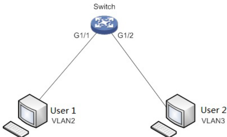
Figure 3-1 VLAN networking
