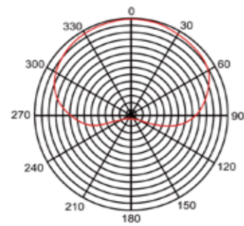
Directivity diagram
