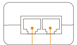
1*100/1000Mbps 802.3af/at PoE+ Output 1*100/1000Mbps Ethernet Data Input
